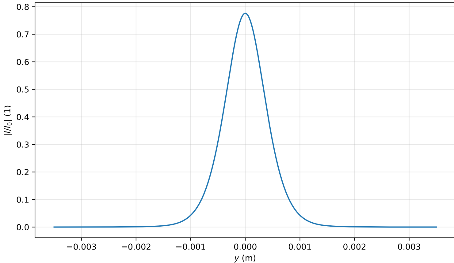
Intensity profile I(x=0, y, z=3.264)/I_0 , P_{in}=0.7P_{cr} , artificial time
